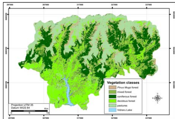
Figure 2. Land cover derived from LANDSAT 7 ETM+ (04.07.2002)
