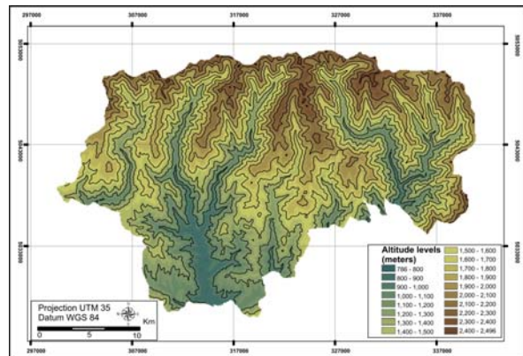
Figure 1. Altitude levels derived from 90 m cell SRTM DEM for Arges basin
