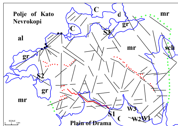
Figure 7. Geological map with the lineaments that mapped by using TM imagery
