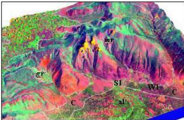
Figure 5. 3D Visualization of Landsat TM image, over the DEM, where: R=PC1, G=PC2 and B=PC3 al: sand, clay, c: conglomerates of marbles, mr: marbles, gr: granodiorite S1: spring Aggitis, W1: well
