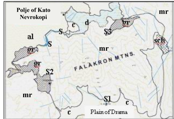
Figure 2. Geological map of the study area, 1:50,000 (IGME) al: Sand, clay, c: conglomerates of marbles, mr: marbles, d: dolomitic marbles, sch: schists, gr: granodiorite, — Faults, — Geological boundary, S1: spring Aggitis, S: sinkholes area
