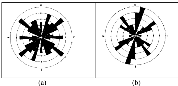
Figure 6. a) Rose diagram of the directions of the map lineaments (Fig. 7).
