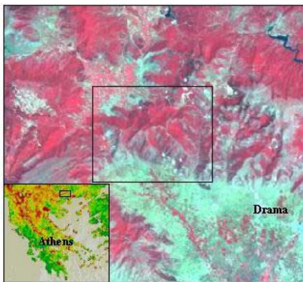
Figure 1. Landsat TM image over the study area. R=band4, G=band2 and B=band1.
