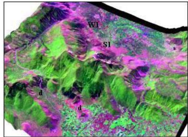
Figure 4. 3D Visualization of Landsat TM image, over the DEM, where: R=band7, G=band4 and B=band2. d: dolomitic marbles, S1: spring Aggitis, WI: well
