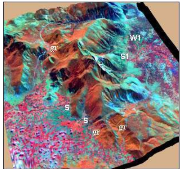
Figure 3. 3D Visualization of Landsat TM image, over the DEM, where: R=band4, G=band5 and B=band2. gr: granodiorite, S1: spring Aggitis, S: shallowholes area, W1: well
