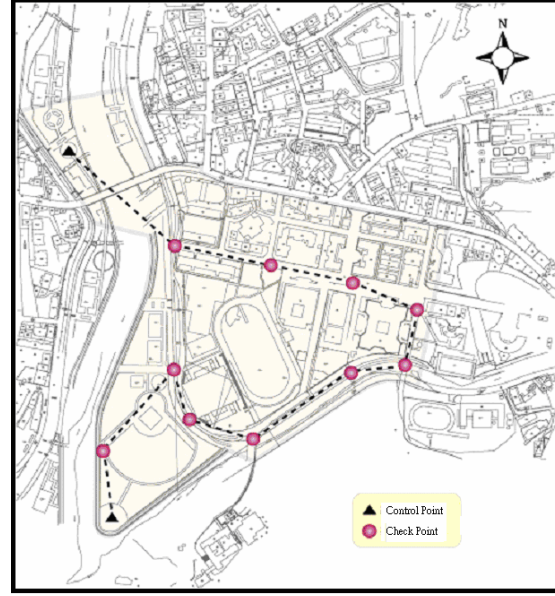
Figure 10. The selected control/check points for RTK/TS test on NCCU campus.
