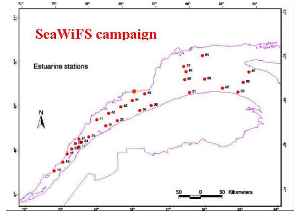
Fig.2 Estuarine stations.
