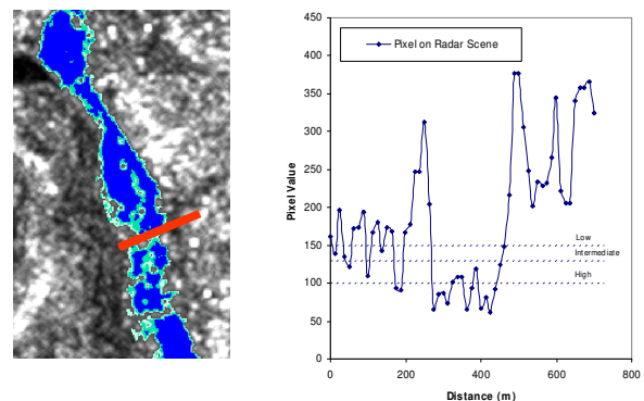
Figure 2. Spectral profile across a river transect
