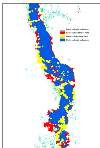
Figure 7. Comparison of the “best” simulation (based on radar observation) and the corresponding Envisat derived flood area
