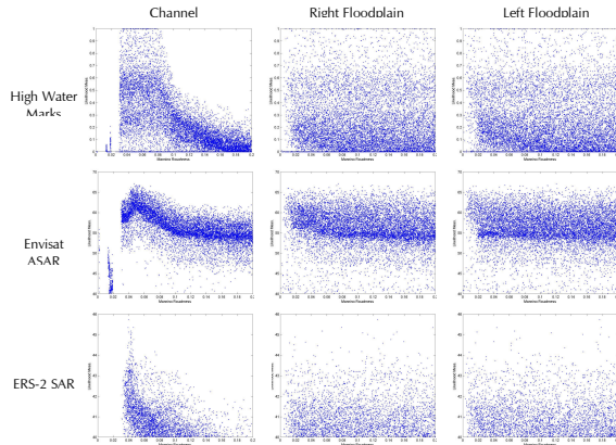
Figure 5 Dotty plots of parameter distributions for the different PMs
