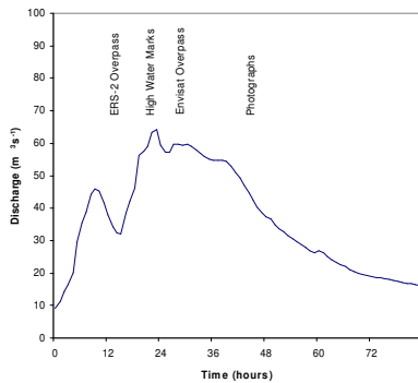
Figure 1. Upstream hydrograph for the 2003 flood event. The satellite overpass times are indicated. The high water marks correspond to the peak flow.
