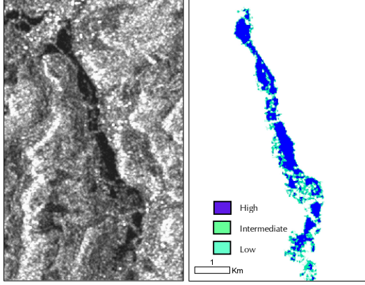
Figure 3. Three probability classes of flooding are defined
