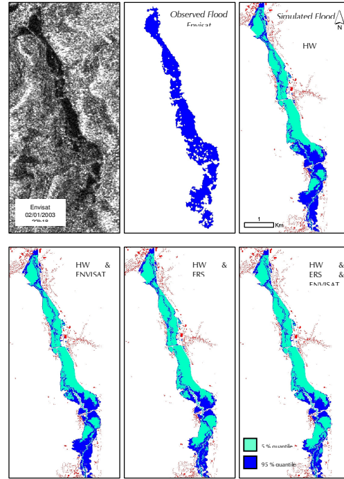
Figure 6. Updated 5% and 95% percentile inundation maps for behavioural simulations of individual and combined PMs (Envisat overpass time)
