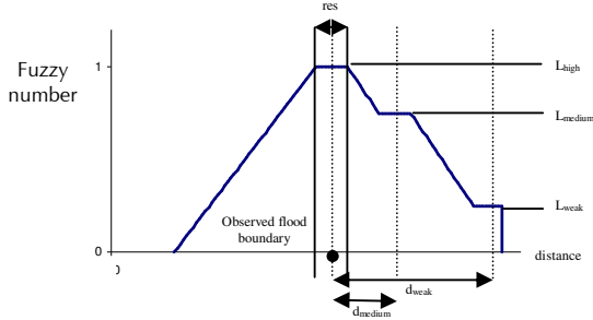
Figure 4. Fuzzy number used in this study
