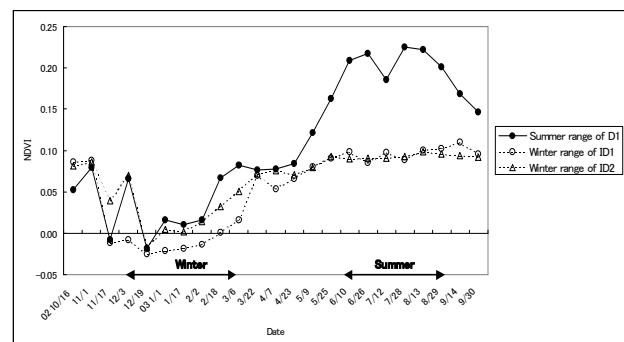
Figure 6. Seasonal changes in NDVI values of the summer and winter ranges in Omnogobi.
