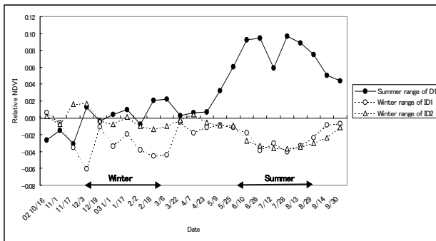
Figure 8. Relative NDVI in the summer and winter ranges, Omnogobi.
