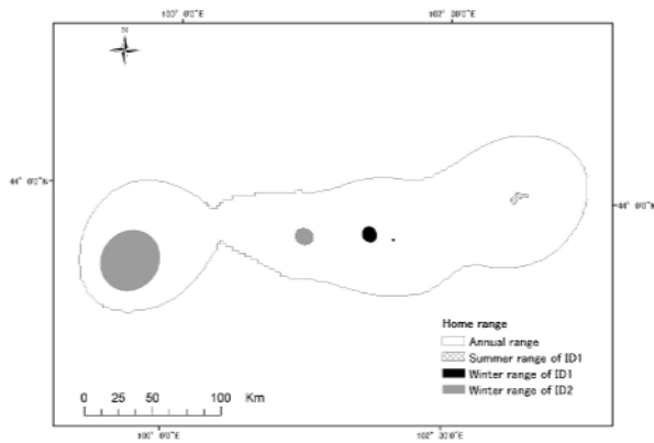
Figure 3. Annual, summer and winter ranges of tracked gazelles in Omnogobi
