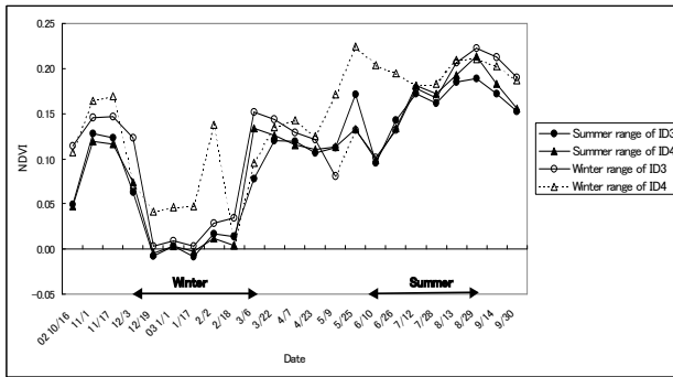
Figure 7. Seasonal changes in NDVI values of the summer and winter ranges in Dornogobi.
