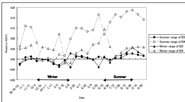
Figure 9. Relative NDVI in the summer and winter ranges, Dornogobi.
