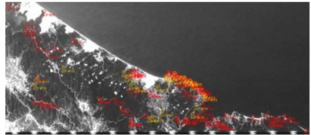
Figure 5. Distribution of GCP's on Corona image
