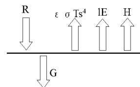
Figure 3. Heat Budget
