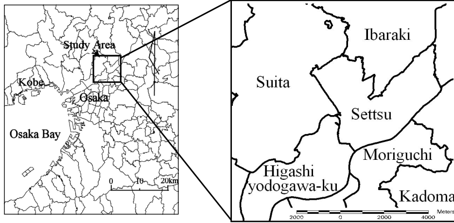
Figure 1. Study area in this research. The area is located in the Kansai district of Japan. It covers 10 km horizontally by 10 km vertically. Five cities and one ward are mainly included in this area.
