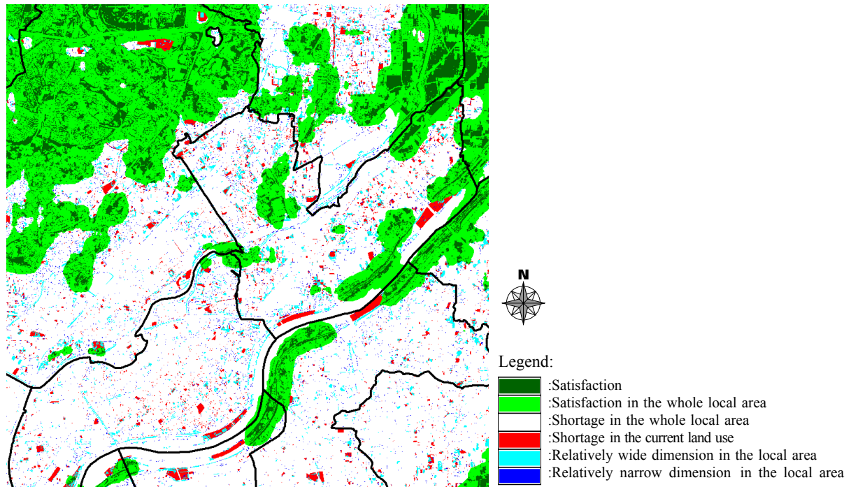
Figure 4. Result of the decision tree method developed in this study. The result contains 6 categories concerned with status of vegetation cover.
