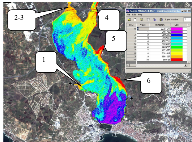
Figure-3 The thematic map of B.Çekmece lake obtained by unsupervised classification showing change in water (Total study area: 2753.63 hectares)
