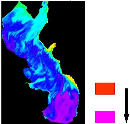
Figure 5: Clearness index map produced from 1 m geometric resolutioned IKONOS image. (The direction of the arrow shows the increase in clearness.)
