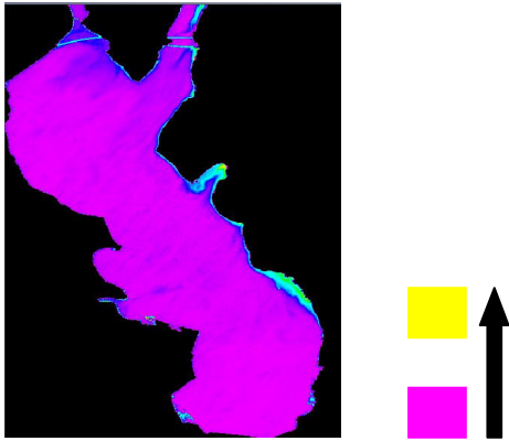
Figure 4: Chlorophyll index map produced from 1 m geometric resolutioned IKONOS image. (The direction of the arrow shows the increase in chlorophyll concentration.)
