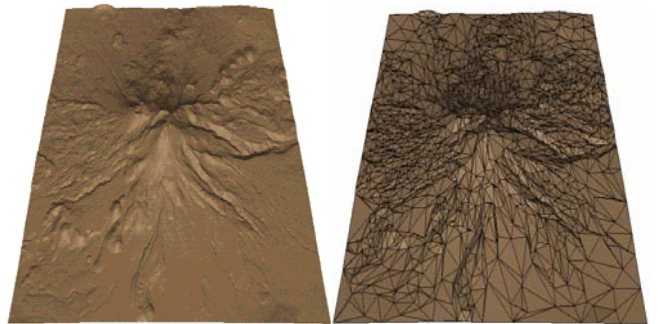
(b) \sigma = 1\varepsilon
