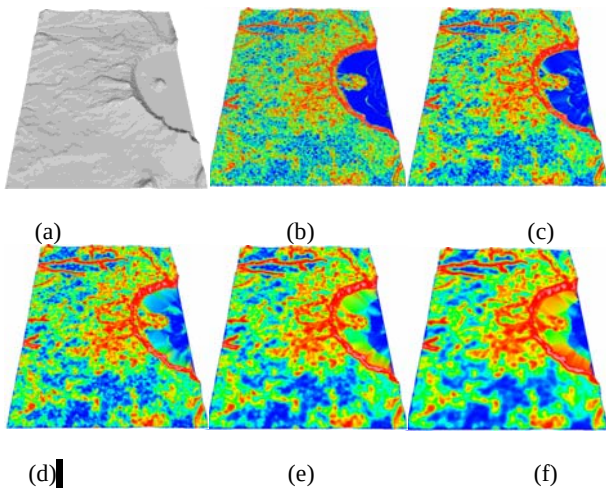
Figure 4: Topographic feature detection: Image (a) shows the “Crater” model, image (b) shows its mean curvature distribution. Images (c) - (f) show the salient features at scales of 1\mathcal{E} , 3\mathcal{E} , 5\mathcal{E} , and 7\mathcal{E} .
