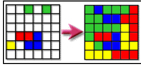
Figure 4. The supervised classification: training sites (left) and the classified image (right). (www.nrca.gc.ca)
