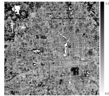
(b) Fraction of vegetation
