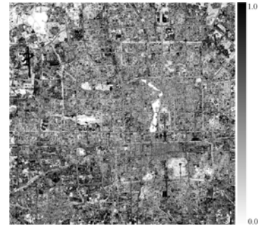
(a) Fraction of manmade materials
