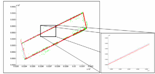
Figure 10. Extracted edge.
