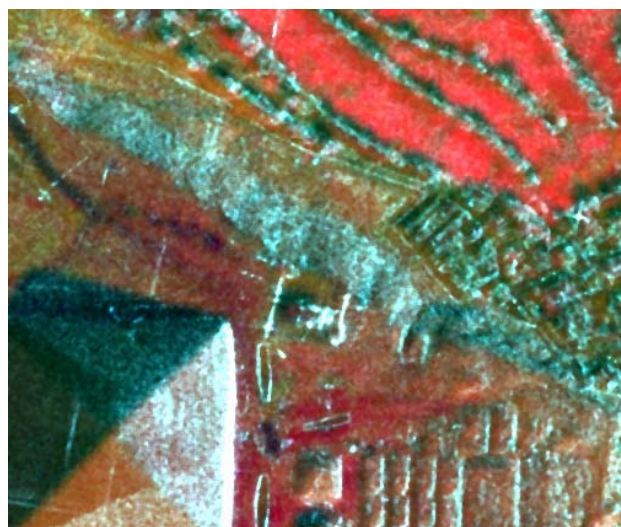
Figure 9: TerraSAR-X fused with Quickbird using PC
