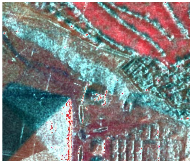
Figure 7: TerraSAR-X fused with Quickbird using Gram-Schmidt
