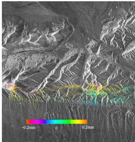
Figure 6 Deformation Levels of the 2329 PS Targets (2004-2006)
