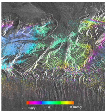
Figure 7 Linear Deformation velocity of the all PSC (after interpolation)
