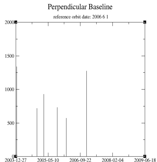
Figure 2. Perpendicular baseline components relative to the selected reference orbit 1-June-2006
