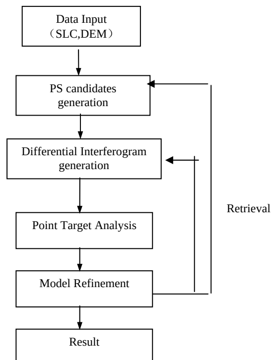
Figure 5. PS Processing Flow Chart
