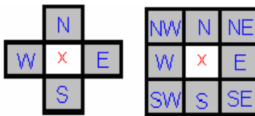
Figure 1 The N_4 and N_8 in 2D raster space
