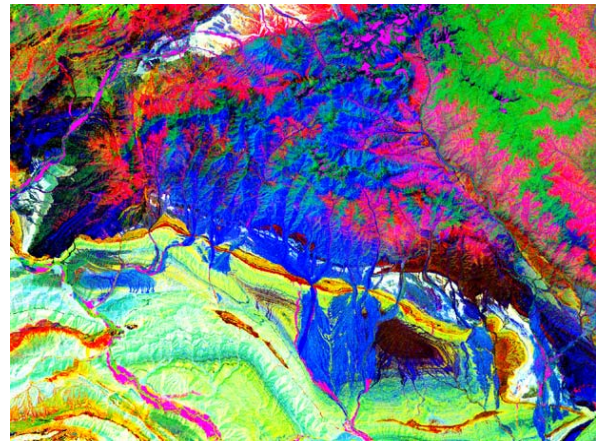
Figure 2 Extraction of ore-control fault (5/8- 4/6-6/7 in RGB)
