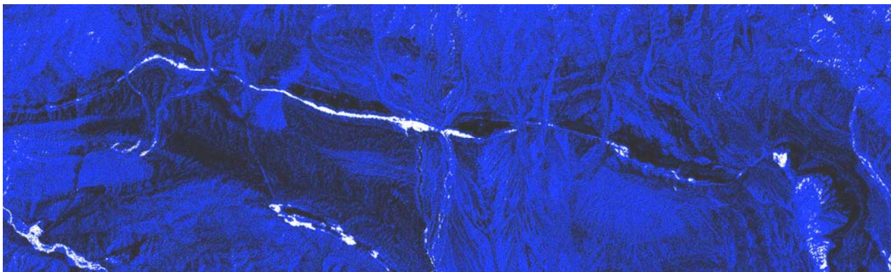
Figure 5 Extraction of alteration information related to \text{OH}^- and \text{CO}_3^{2+}
