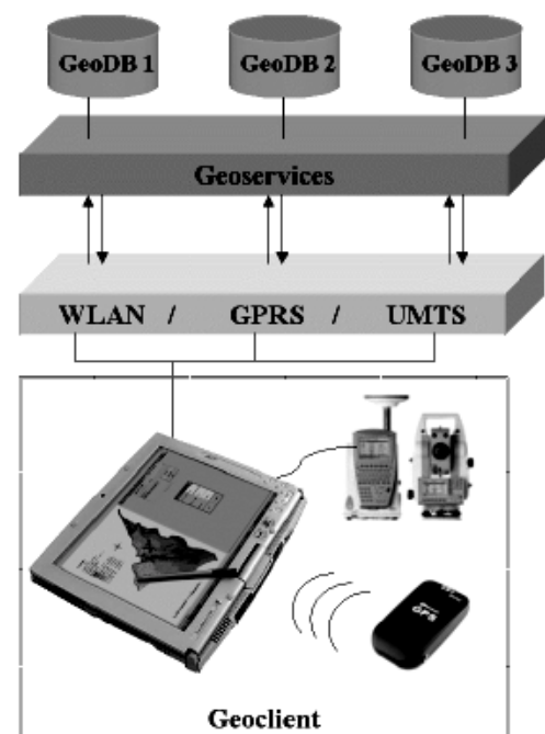
Figure4. Field based Mobile GIS architecture
