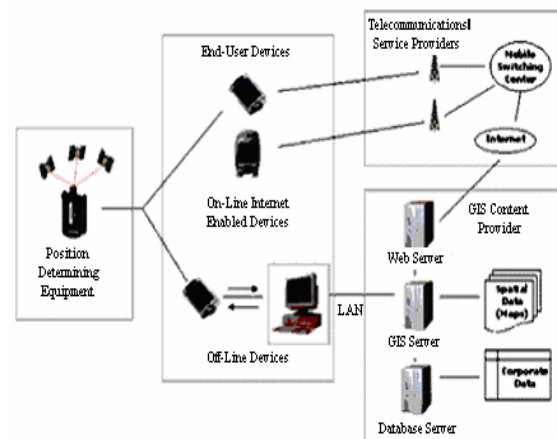
Figure3. Components of Mobile GIS
