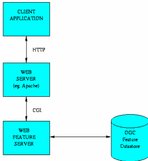
Figure2. WFS architecture
