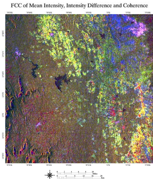
Fig 3: FCC of mean intensity (Red), intensity difference (Green) and coherence image (Blue)
