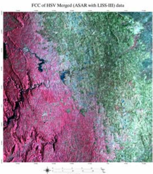
Fig 5: FCC of IHS merged (ASAR with LISS-III) data
