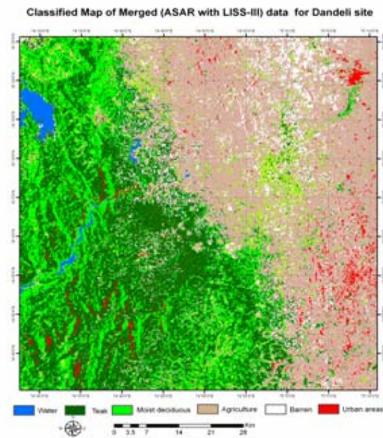
Fig 6: Vegetation classified map of IHS merged data
