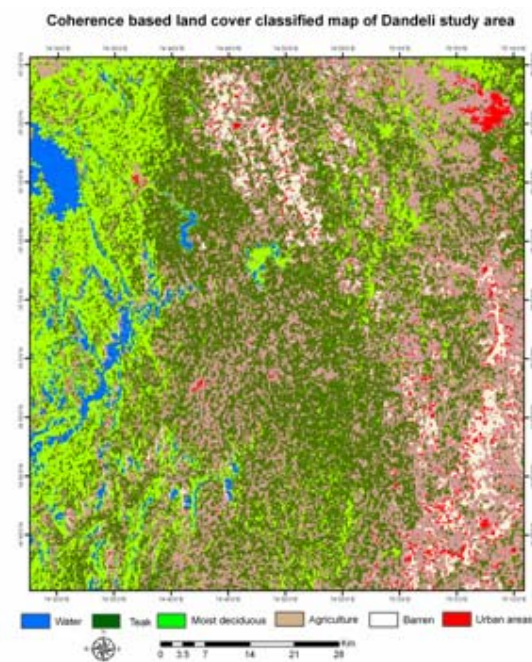
Fig 4: Vegetation type classified map generated from FCC of mean intensity, intensity difference and coherence image
