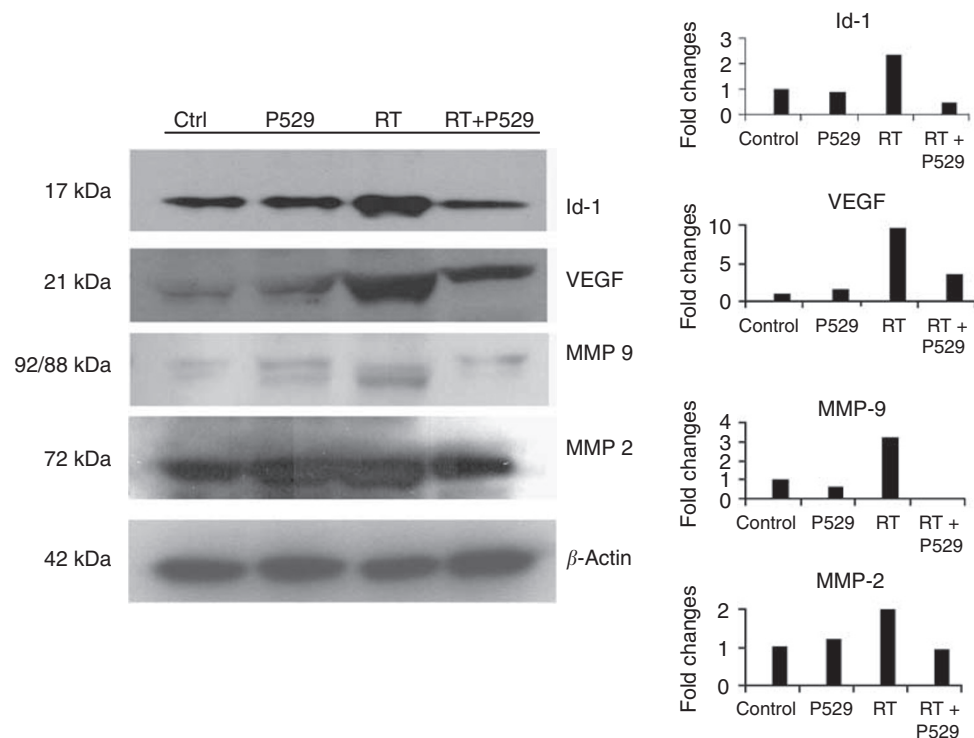
Figure 4 Effect of P529, ionising radiation, and the combination of both treatments on Id-1, VEGF, MMP-9, and MMP-2 protein levels. Amount of Id-1 is increased by RT, but addition of P529 reduces Id-1 below control levels. The combination RT + P529 also decreases RT-induced VEGF levels. Active MMP-9 is reduced in RT-treated cells by the addition of P529. Levels of active MMP-2 are also decreased by the addition of P529 to RT-treated cells. In the densitometric analysis, the Y-axis represents fold changes with respect to control.
