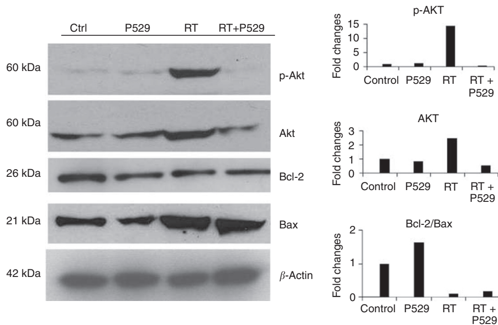
Figure 3 Effect of P529, RT, and P529 + RT and the combination on p-Akt, total Akt, Bcl-2, and Bax. Ionising radiation causes a > 10-fold increase in p-Akt levels. However, when P529 is added to the treatment, p-Akt levels are lower than those observed in untreated cells. Total Akt levels are also increased in RT-treated cells, but levels return to normal when the drug is added. Bcl-2 decreases as a consequence of P529, RT, and combination treatment, whereas Bax increases in RT- and RT + P529-treated cells. The densitometric analysis shows that the Bcl-2/Bax ratio is reduced in RT and RT + P529 cells. The Y-axis represents fold changes with respect to control.
