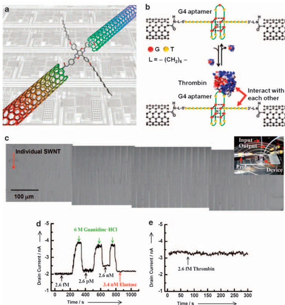
Figure 4 (a) Schematic of single-molecule devices using SWNT point contacts. Adapted from Feldman et al. 70 (© 2008 ACS). (b) Schematic representation of the sensing design showing how single-molecule devices can detect proteins at the single-molecule level. (c) Scanning electron microscopy images showing highly integrated identical SWNT devices. Inset shows an optical image of a single-molecule device during real-time measurements. (d) Current-versus-time data recorded for an aptamer-rejoined device upon alternate additions of the thrombin Tris-HCl buffer solution at different concentrations (from 2.6 fM to 2.6 pM and 2.6 nM), the 6-M guanidine HCl solution, and finally the elastase (3.4 nM) Tris-HCl buffer solution. (e) I - V plot recorded for a Con-A-rejoined device upon injection of 2.6 fM thrombin in Tris-HCl buffer solution. All the measurements were performed at V_D = -50 mV and V_G = 0 V. Adapted from Liu et al. 71 (© 2011 Wiley-VCH).
