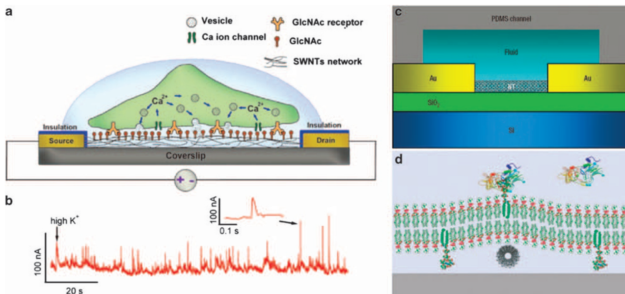
Figure 1 (a) Triggered exocytosis and SWNT-net detection. (b) Nanotube responses to exocytosis of PC12 cells triggered by high K^+ stimulation. The SWNT-net was biased at V_{ds}=0.4 V. Adapted from Sudibya et al. 57 (© 2009 Wiley-VCH). (c) Schematic of the side view of a SWNT FET inside a polydimethylsiloxane (PDMS) microfluidic channel. (d) Scaled schematic of a carbon nanotube under a 1,2-dioleoyl-sn-glycero-3-phosphocholine (DOPC) bilayer. The DOPC lipid molecules are shown with two light green fatty acid chains. A toxin protein, represented in a ribbon model, binds to a membrane-embedded ganglioside molecule that is shown with two dark green chains. Adapted from Zhou et al. 60 (© 2007 NPG).
