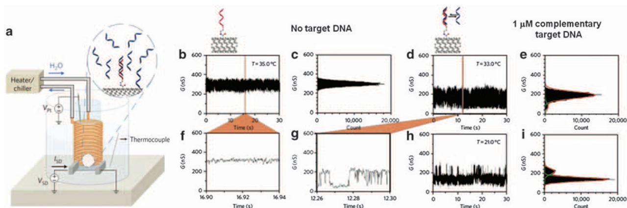
Figure 3 (a) Schematic of the nanotube device used for studying the kinetics and thermodynamics of DNA hybridization (with an external circular heater/refrigerator to control temperature). (b, d, h) Conductance recordings of devices over one 30-s interval with DNA oligonucleotide probe \text{H}_2\text{N} -5'-GGAAAAAGG-3' without exposure to complementary DNA target at 35.0 °C (b), after exposure to complementary DNA target at 33.0 °C (d) and after exposure to complementary DNA target at 21.0 °C (h). The source-drain bias is 100 mV and V_{\text{Pt}} is zero. (c, e, i) Conductance-based histograms of time intervals shown in b, d and h. The two levels in e and i are fit to the Gaussian distributions. (f, g) Representative short time interval (40 ms) for real-time conductance recording for probe only and after exposure to complementary target DNA. Adapted from Sorgenfrei et al. 68 (© 2011 NPG).
