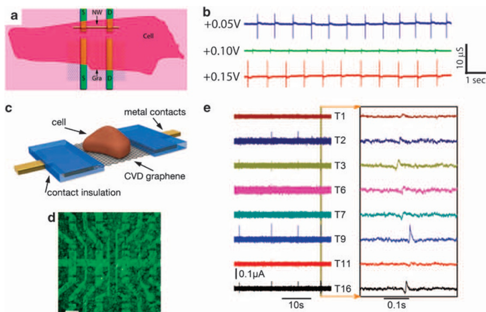
Figure 7 (a) Representation of the relative size of cardiomyocyte cell interfaced to typical Graphene and silicon nanowire-FET devices. (b) Recorded traces at different applied water gate potentials. The following blue, green and red traces were recorded at +0.05, +0.10 and +0.15 V, respectively. The corresponding sensitivities are 2020, 398 and 2290 \mu\text{S V}^{-1} , respectively. Adapted from Cohen-Karni et al. 83 (© 2010 ACS). (c) Schematic view of a graphene FET with a cell on the gate area. The graphene is shown between the drain and source metal contacts, which are protected by a chemically resistant layer. (d) Combination of an optical microscopy image of a transistor array and a fluorescence image of the calcein-stained cell layer on the same array. The scale bar is 100 \mu\text{m} . (e) Simultaneous current recordings of eight transistors in one FET array over tens of seconds (left) and hundreds of milliseconds (right). Adapted from Hess et al. 84 (© 2011 Wiley-VCH).
