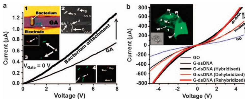
Figure 5 (a) The conductivity of the p-type GA device increases upon attachment of a single bacterial cell on the surface of GA (the device is shown in inset 1). (b) DNA transistor: single-stranded DNA (ssDNA) tethering on GO increases the conductivity of the device. Successive hybridization and dehybridization of DNA on the G-DNA device results in completely reversible increase and restoration of conductivity. Inset shows a G-DNA(ds) sheet with wrinkles and folds clearly visible. Adapted from Mohanty et al. 72 (© 2008 ACS).
