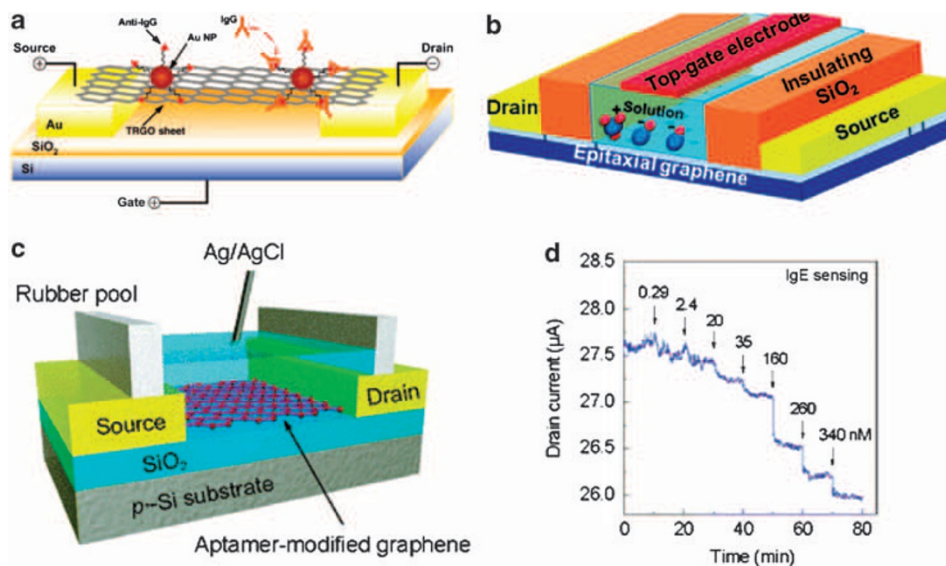
Figure 6 (a) Schematic of a reduced GO FET. Anti-immunoglobulin G (IgG) was anchored to the reduced GO sheet surface through Au nanoparticles and functions as a specific recognition group for the IgG binding. Adapted from Mao et al. 74 (© 2010 Wiley-VCH). (b) Schematic illustration of the device structure for solution-gated graphene FETs. Adapted from Ang et al. 77 (© 2008 ACS). (c) Schematic illustration of aptamer-modified electrolyte-gated graphene FETs. (d) Time course of ID for an aptamer-modified graphene FET. At 10-min intervals, various concentrations of IgE were injected. Adapted from Ohno et al. 79 (© 2010 ACS).
