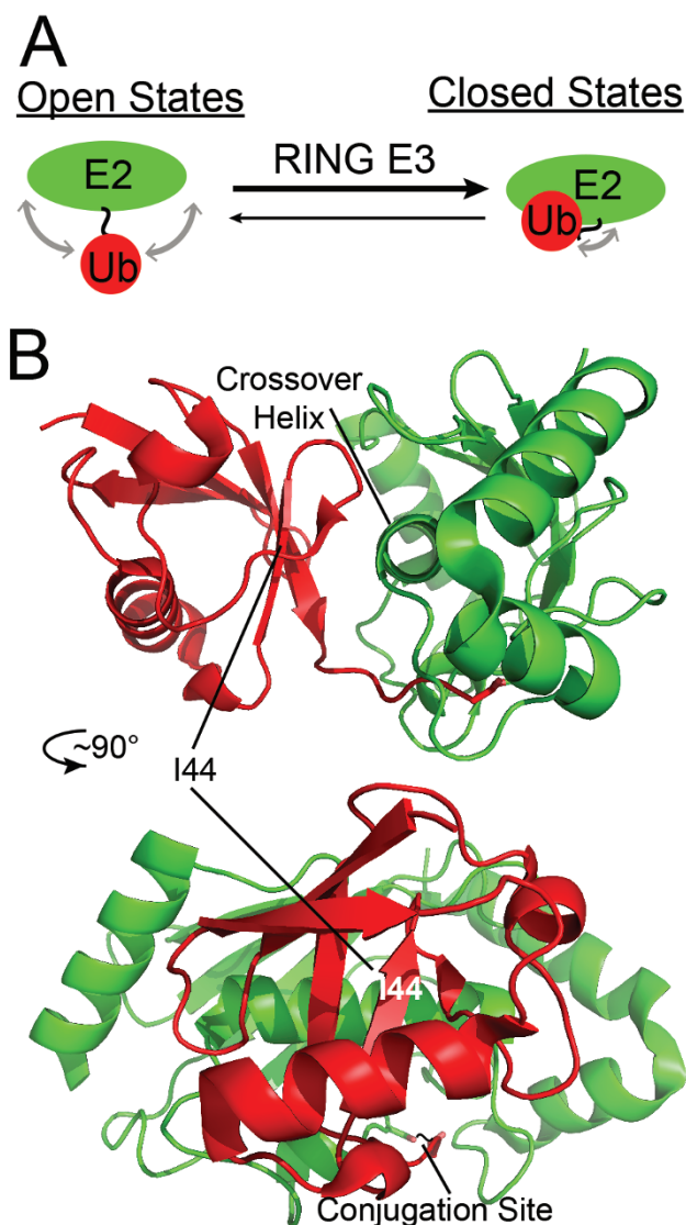
Figure 2 Ubiquitin positioning in the E2~Ub conjugate. (A) A cartoon depiction of the dynamic “open states” in which Ub samples a range of various positions relative to the E2, but shifts towards population of more “closed states” upon binding of a RING-type E3. (B) Crystal structure of an E2~Ub oxyester conjugate (Ube2D2) in a closed state showing the interface formed between the E2 (green) crossover helix and the I44 surface of Ub (red) upon binding a RING E3 (BIRC7 (not shown); PDBID: 4AUQ). The two representations are the same structure rotated ~90° about the vertical axis. The E2 is in the same orientation as in Figure 1 in the bottom representation.
