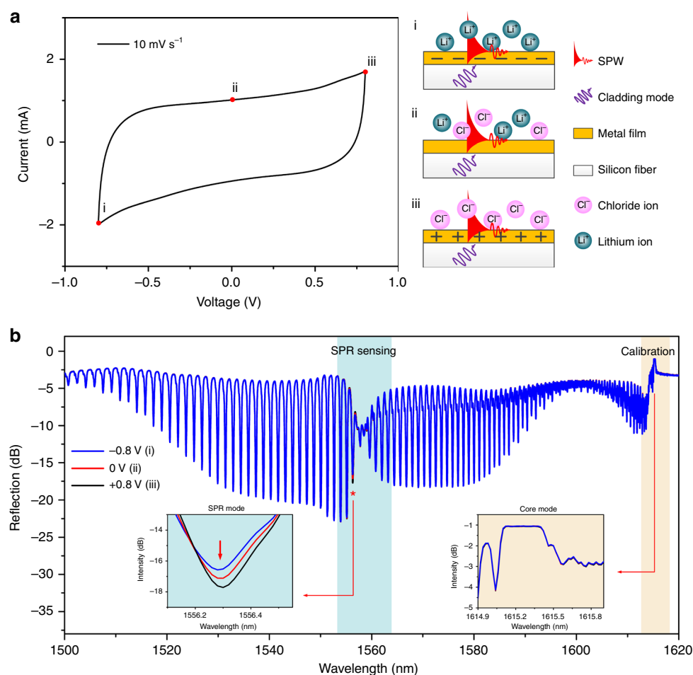
Fig. 1 Electrochemical surface-plasmon-resonance sensing principle and experimental demonstration with an gold-coated TFBG optical fiber sensor. a CV response of the supercapacitor during a polarizing cycle including positive and negative polarities, and the resulting electronic polarizations of Au film: (i and iii) two opposite polarizations at -0.8 V and +0.8 V; (ii) neutral state ( 0 V). b Spectral response of P-polarized input, gold-coated 18^\circ TFBG for the different electronic polarization states of the electrode; enlarged view (blue inset) of the spectral change of the SPR coupled cladding mode used for monitoring (marked by a red asterisk “*”); and (yellow inset) enlarged view of the spectrum near the core mode (Bragg) reference resonance
