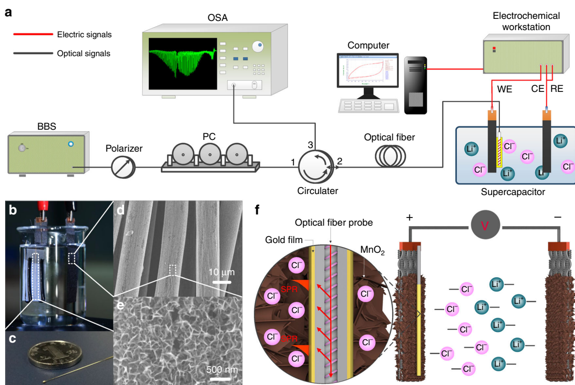
Fig. 5 Electrochemical surface-plasmon-resonance sensing principle and experimental demonstration with a gold-coated TFBG optical fiber sensor. a Experimental setup of a plasmonic fiber-optic sensing system for monitoring the SOC of supercapacitors. b Photographs of the configuration for the supercapacitor and (c) gold-coated fiber-optic sensing probe. SEM images of (d) the \text{MnO}_2 electrode and (e) the corresponding magnified image. f Schematic of the measurement of the charge-discharge process of supercapacitors by a plasmonic gold-coated TFBG fiber-optic sensor
