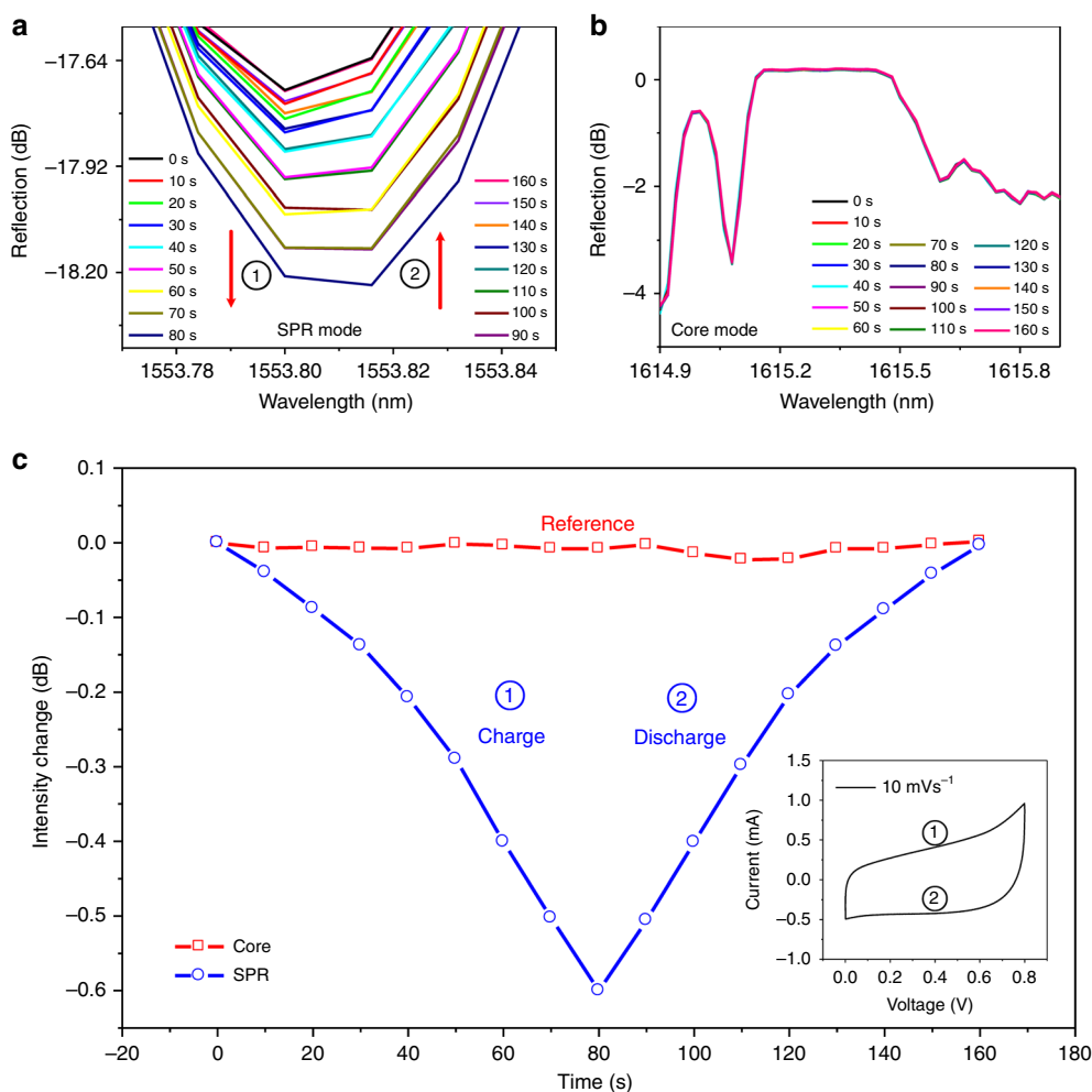
Fig. 2 Detailed charging and discharging of the supercapacitor from 0 to 0.8 V. a Spectral response of the selected SPR resonance (the red arrow indicates the variation trend of the SPR spectral feature with time) and (b) unchanged core Bragg resonance. The electrochemical curve and the optical response are synchronously recorded. c Intensity change of the selected SPR resonance (blue dot) and the core Bragg resonance (red block) corresponding to one cycle of the CV curve of the supercapacitors at a scan rate of 10 mV s -1 (shown in the inset). The symbol ① represents the process of charging. Conversely, the symbol ② represents the process of discharging
