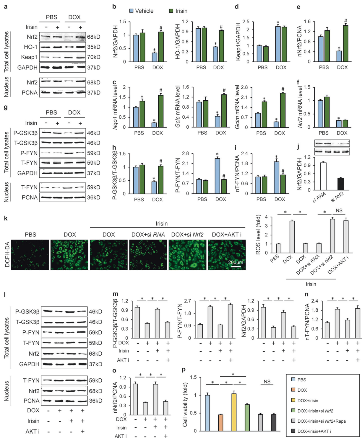
Fig. 6 AKT/GSK3β/FYN/Nrf2 signaling was responsible for FND5C5-mediated protective role on oxidative damage. a, b Western blots and statistical results ( n = 6 ). c Relative mRNA levels of Nqo1 , Gclc , and Gclm in cultured H9C2 cells ( n = 6 ). d, e Keap1 protein levels in total cell lysates and Nrf2 protein levels in nuclear lysates ( n = 6 ). f Relative Nrf2 mRNA level ( n = 6 ). g, h Representative western blots ( n =
