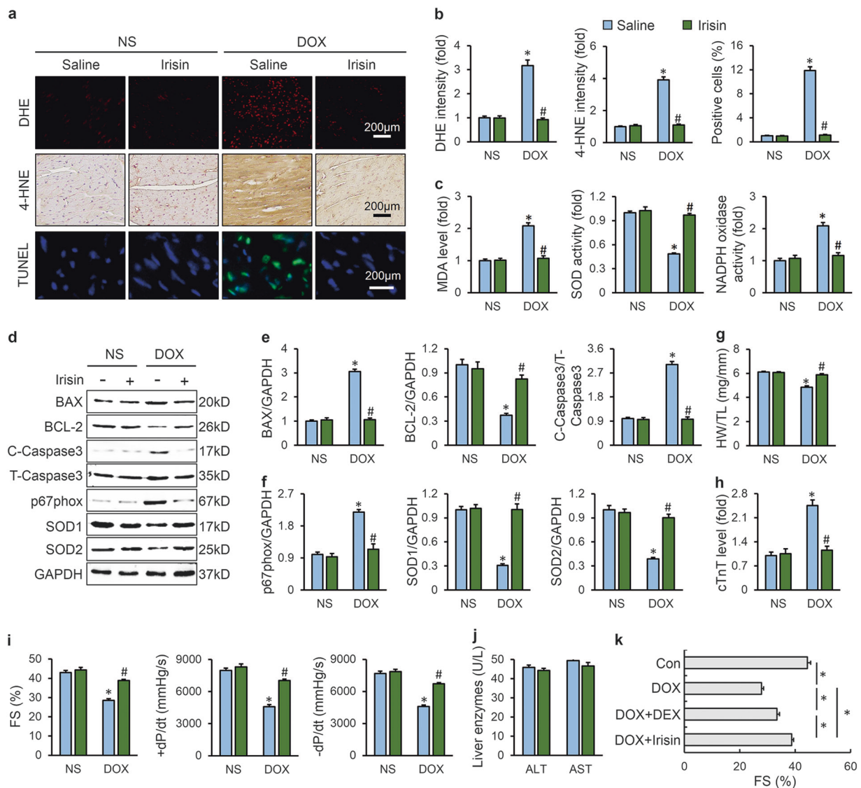
Fig. 8 FNDC5/Irisin was a potential therapeutic agent against DOX-induced cardiotoxicity. a, b Representative DHE, 4-HNE, TUNEL staining images and statistical results ( n = 6). c Quantitative results of myocardial MDA levels and SOD, NADPH oxidase activities ( n = 6). d-f Western blots and statistical results ( n = 6). g Statistical results of the heart weight/tibia length (HW/TL) ( n = 8). (h) Serum cTnT levels
