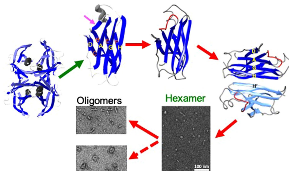
Figure 5. Proposed molecular mechanism of TTR aggregation on the basis of our biochemical analyses and previous experimental results. Under amyloidogenic conditions, tetrameric native TTR is dissociated to monomers, which undergo local conformational changes in AB loop region (pink arrow) 31 . The amyloidogenic monomers form a dimer through H-H' interactions. The dimers are then associated to form spherical hexamers, which self-assemble into linear (WT TTR) or annular oligomers (G53A). The structural models for the native tetramer, monomers, and dimers were drawn using MOLMOL 60 with pdb code (1F41) 61 .
