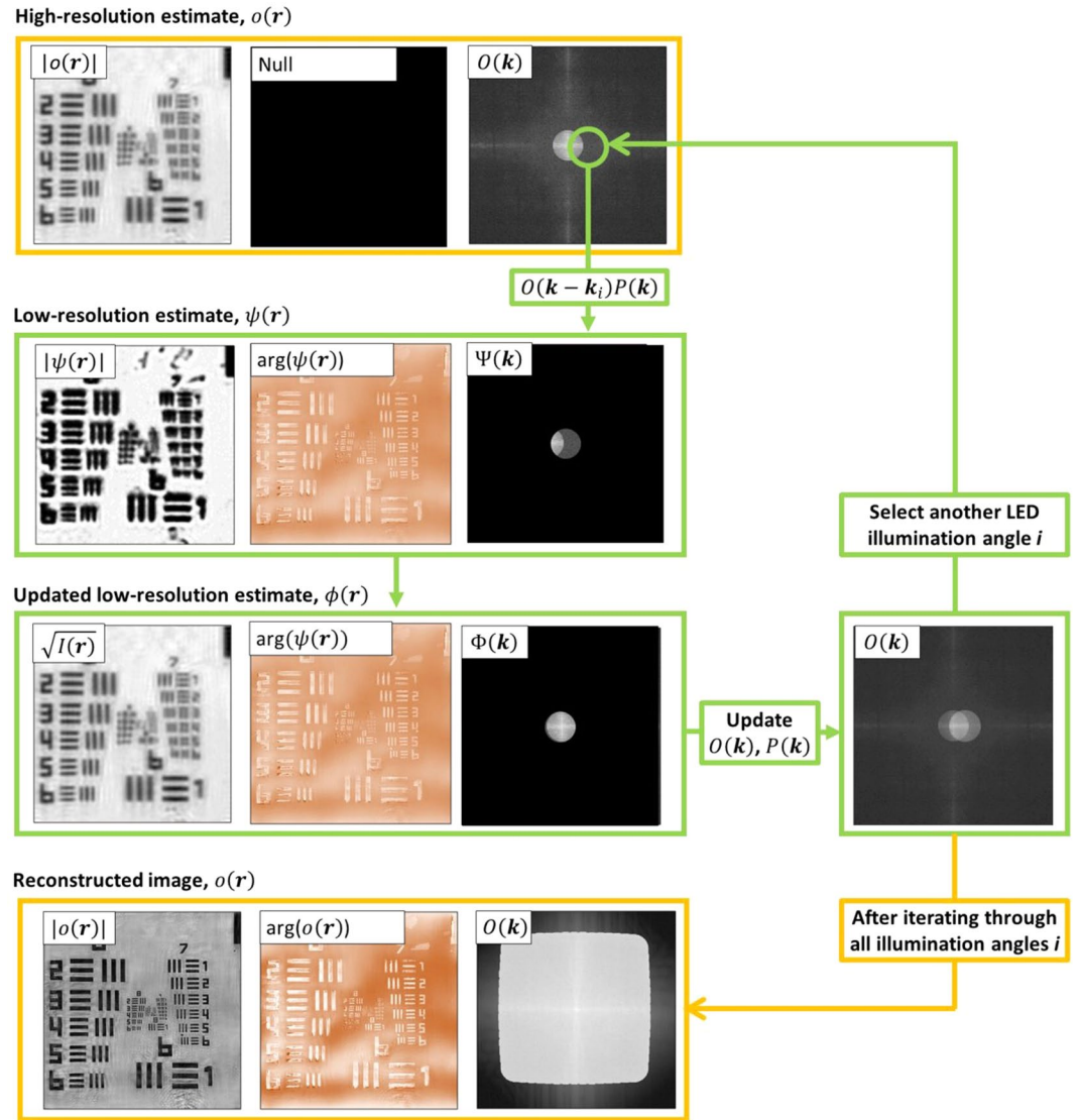
Figure 5. Diagram of a single FPM reconstruction algorithm iteration n . It starts by initializing a high-resolution image estimate o_0(r) , which was an interpolated experimental brightfield image. For each illumination angle, a region of the high-resolution estimate spectrum, corresponding to illumination angle i is low-pass filtered to produce an estimate of the low-resolution image: \psi_n^{(i)} . A new estimate, \phi_n^{(i)} is obtained by replacing the amplitude of \psi_n^{(i)} with the amplitude of the demosaiced recorded image, \sqrt{I} , while retaining the phase of \psi_n^{(i)} . The low-resolution spectrum is added into the high-resolution spectrum using eqs (6) and (7) to yield the updated object spectrum and pupil functions O_{n+1}(k) and P_{n+1}(k) . The whole process continues till spectrum regions corresponding to all illumination angles are updated. An example of the reconstructed spectrum is shown at the bottom of the figure.
