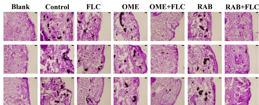
Figure 3. Histopathology of infected G. mellonella larvae treated with different drugs. After infection with CA10 ( 5 \times 10^8 CFU/mL), larvae were treated with PBS, FLC (160 \mu g/mL), OME (80 \mu g/mL), RAB (40 \mu g/mL), OME (80 \mu g/mL) plus FLC (160 \mu g/mL) or RAB (40 \mu g/mL) plus FLC (160 \mu g/mL). The larvae of the blank groups were not treated with yeast or any drugs. Tissue sections were observed at a 4.2 \times 10 multiplier, with a scale of 20 \mu m.
