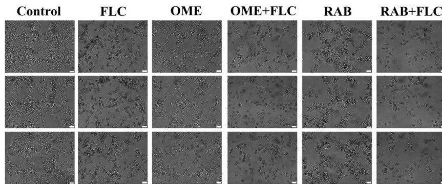
Figure 4. Effects of PPIs combined with FLC on the morphologic transformation of resistant C. albicans . A yeast suspension ( 5 \times 10^5 CFU/mL) was incubated in RPMI-1640 medium with PBS, FLC (8 \mu g/mL), OME (128 \mu g/mL), OME (128 \mu g/mL) plus FLC (8 \mu g/mL), RAB (64 \mu g/mL) or RAB (64 \mu g/mL) plus FLC (8 \mu g/mL). After an incubation of 5 h at 35 °C, cells were observed under an inverted microscope at a 40 \times 10 multiplier, and the scale in the figure is 20 \mu m.
