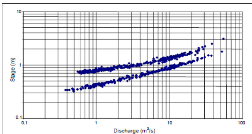
Figure 3: Koga at Wetet Abay - Discharge Measurement
