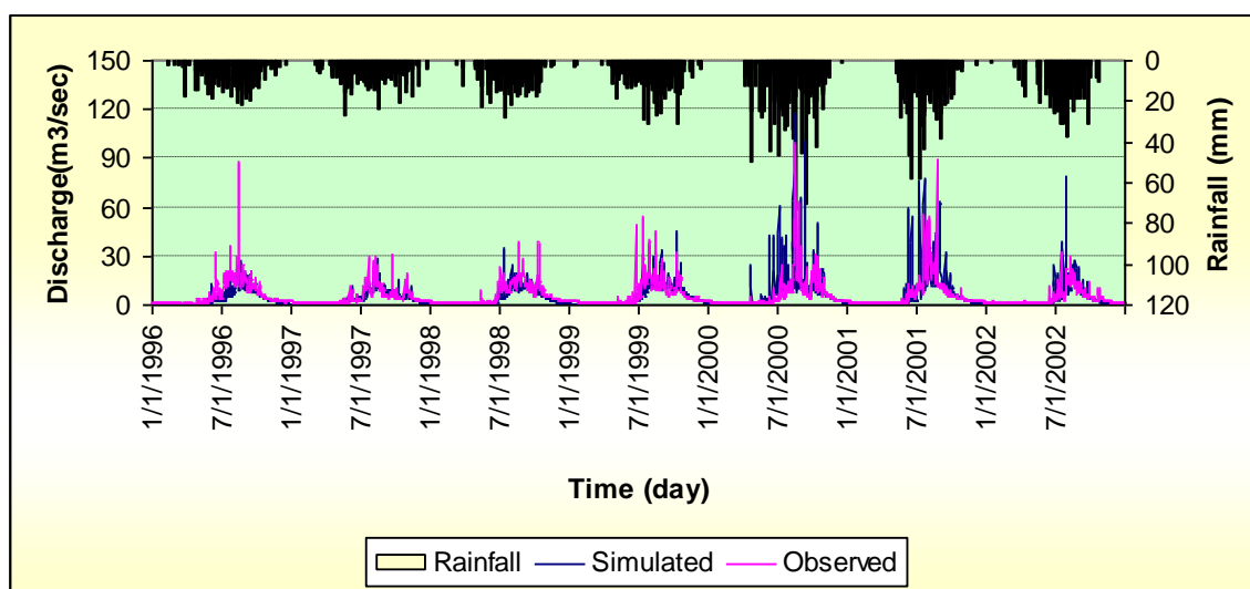
Figure 10: Daily flows during calibration period for Koga subcatchment
