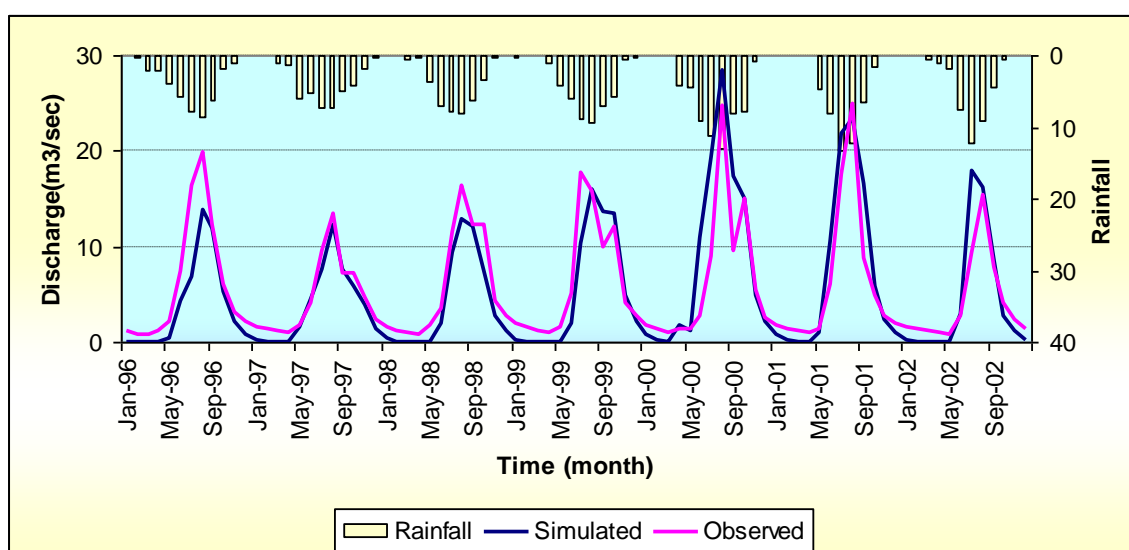
Figure 11: Monthly flows during calibration period for Koga subcatchment
