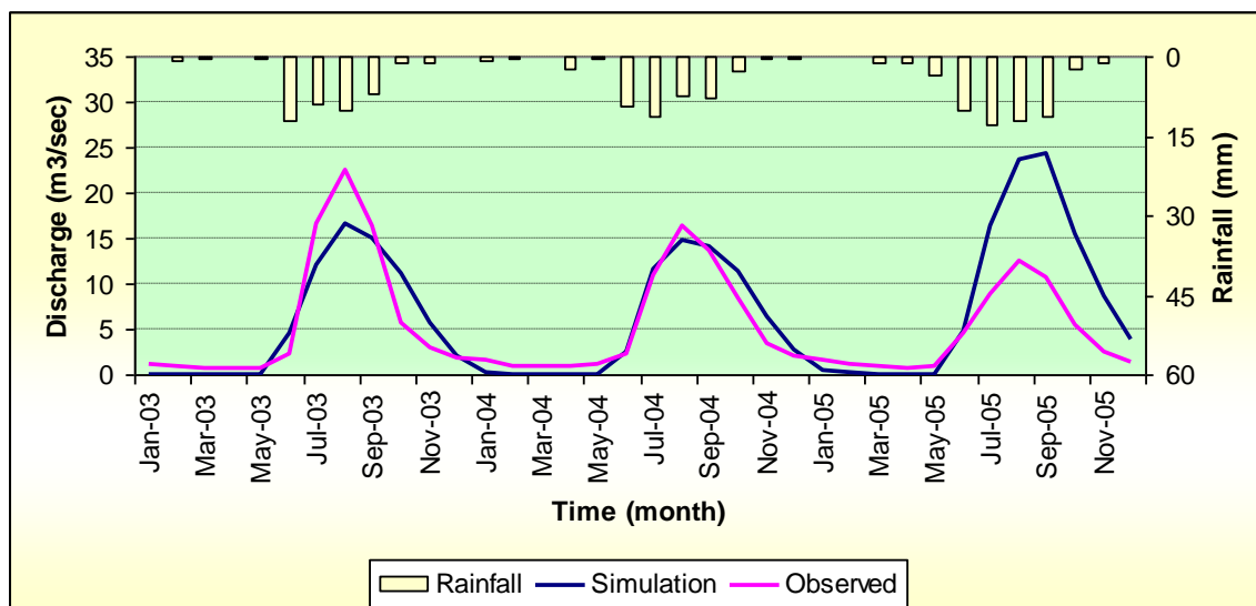
Figure 13: Monthly flows during verification period for Koga subcatchment
