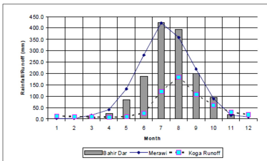
Figure 2: Comparison of Bahir Dar and Merawi Rainfall and Koga River Flows
