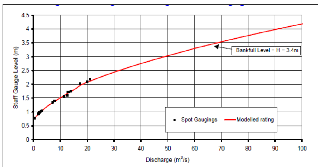
Figure 4: Rating curve at the Dam Site
