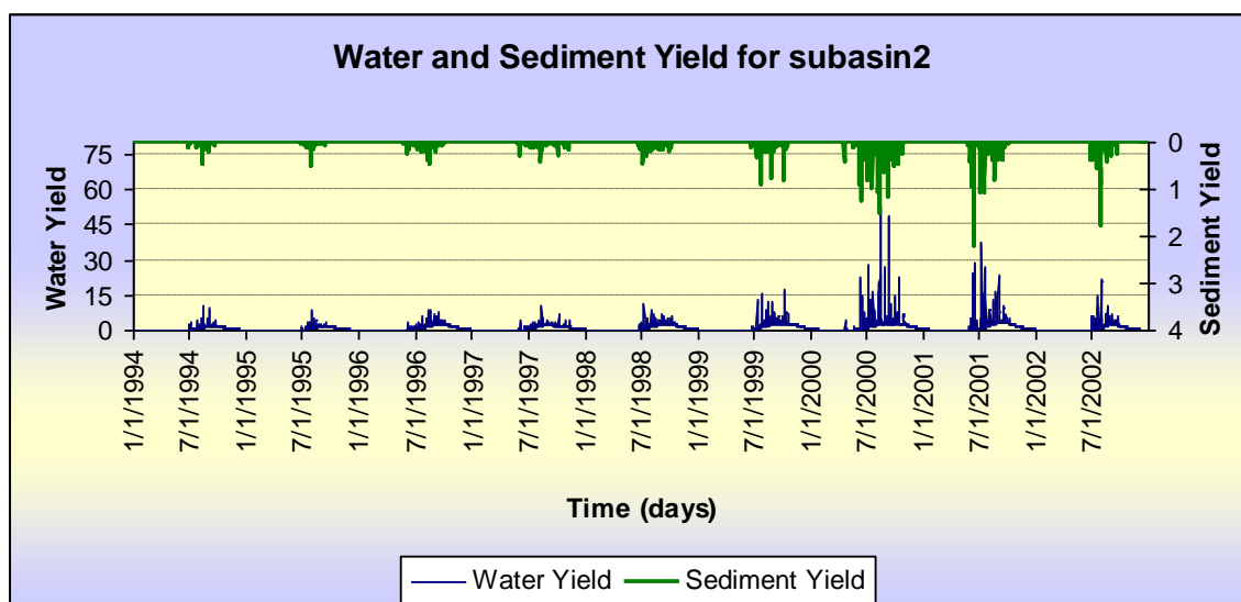
Figure 15: Water and Sediment Yield at the outlet of Subbasin 2
