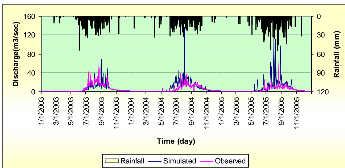
Figure 12: Daily flows during verification period for Koga subcatchment
