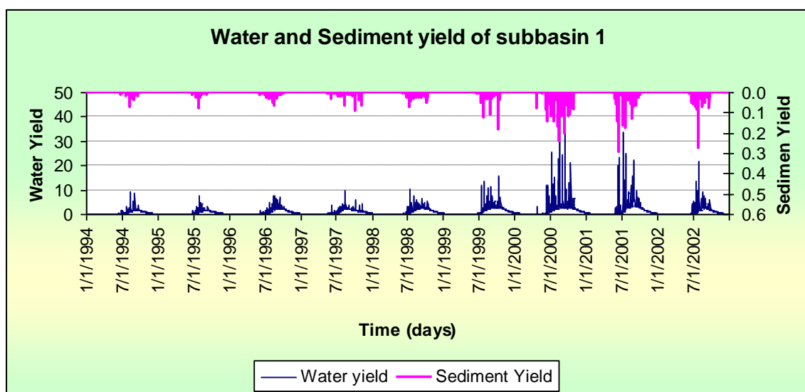
Figure 14: Water and sediment yield at the outlet of subbasin 1
