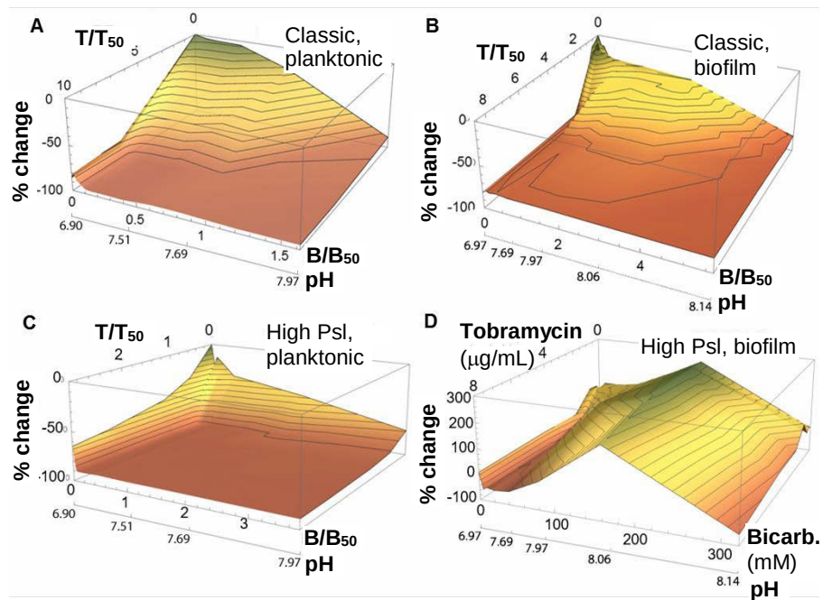
Figure 2.2 We use response surfaces to measure the effect of tob and bicarbonate (bicarb) combinations on (A,C) planktonic bacteria and (B,D) biofilms of (A,B) a CF clinical isolate with “classic” phenotype and (C,D) a CF isolate with high Psl. (A-C) Tob and bicarb concentrations are plotted as the fraction of the concentration corresponding to 50% inhibition of growth ( \text{MIC}_{50} ). (D) \text{MIC}_{50} is not well-defined for this system, so actual concentrations are used. (A,C) The planktonic response surfaces are concave-upward, reflecting synergy between tob and bicarb. (B,D) The biofilm response surfaces are concave-downward, reflecting antagonism between tob and bicarb. (C,D) The high-Psl isolate shows greater antagonism in the biofilm state than does the classic isolate, even though the high-Psl isolate shows greater synergy in the planktonic state. (D) Portions of the biofilm response surface extend above 0% change, indicating that treatment has enhanced biofilm activity. All panels from [13].
