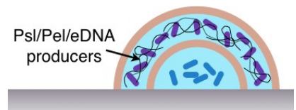
Figure 2.4: Bacterial microenclosure.
