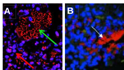
Figure 3.1. P. aeruginosa biofilm aggregates surrounded by neutrophils (A) in a CF lung [1] and (B) in a chronic wound [12]. Bacterial aggregates (red, green and white arrows) are surrounded by neutrophils (blue, red arrow).
