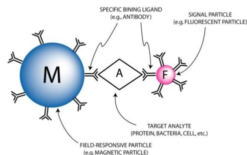
Figure 2. Particle complex approach to sandwich immunoassays. The magnetic particle provides concentration and specific signal enhancement. The fluorescent particle provides signal amplification.
