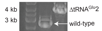
Figure 12. PCR gel confirming chloramphenicol resistance gene (CAT) replaced tRNA Glu2 .
