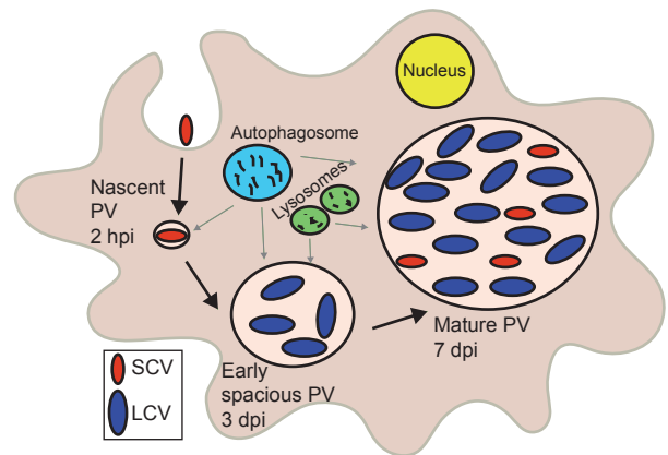
Figure 1. Biogenesis of C. burnetii parasitophorous vacuole (PV).
