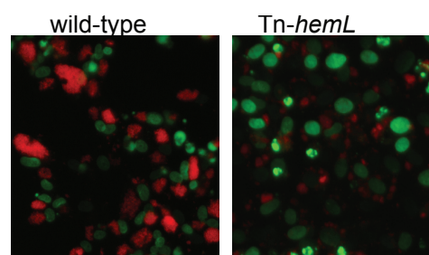
Figure 8. Tn insertion in hemL reduced intracellular growth significantly. Host nuclei shown in green and C. burnetii PVs in red. Data from Martinez et al. 2014.
