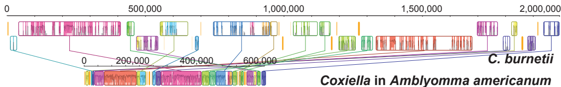
Figure 5. Alignment of Coxiella genomes. Regions in white in C. burnetii genome (on top) denote genes present only in the human pathogen. Modified from Smith et al. 2015. specific genes ( Figure 5 ). We will also use reciprocal BLAST, as described previously (Raghavan et al. 2012; Raghavan et al. 2015; Smith et al. 2015) to identify pathogen-specific genes i.e. C. burnetii genes without orthologs in tick associated Coxiella . By comparing the C. burnetii genomes, we will identify pathogen specific metabolic genes that are conserved in all strains of C. burnetii .
