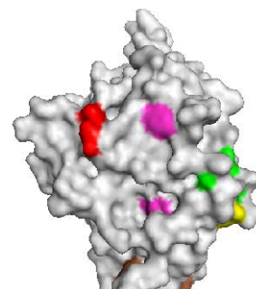
Positions on HSV gD targeted by a few different antibodies.
