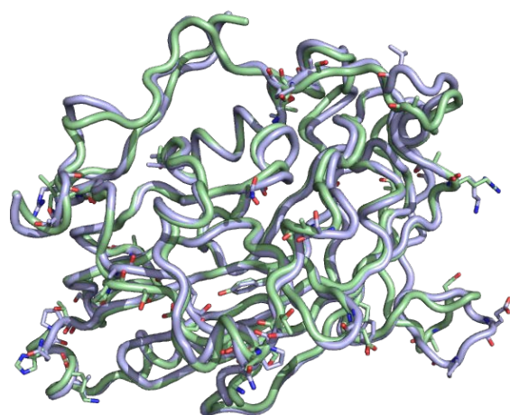
Figure C.2. Superposition of gD1 structure and gD2 homology model, with backbones in ribbon mode and side chains shown only for positions with different amino acids.
