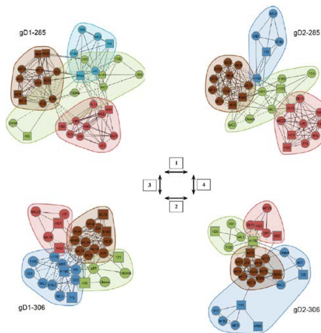
Figure C.3. Antibody community maps from four gD variants. A community plot is a network plot (e.g. social networks) generated from the epitope binning heat maps. The different colors represent 4 Wasatch derived unique communities formed by the binning characteristics of 40 different gD monoclonal antibodies obtained from 6 different laboratories. Circles represent binding in both directions (surface attached and in solution) whereas squares represent binding only in one direct. Chord length indicates degree of relatedness as defined by relative completion in the binning assay. Dashed chord indicate that there is asymmetry in the relationship (i.e. blocking does not reciprocate).
