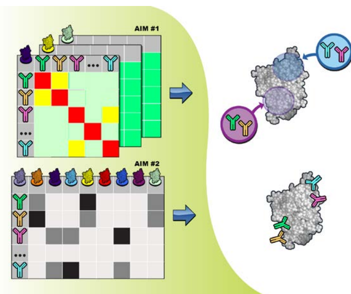
Figure C.1. Cartoon intuition for the approaches.
