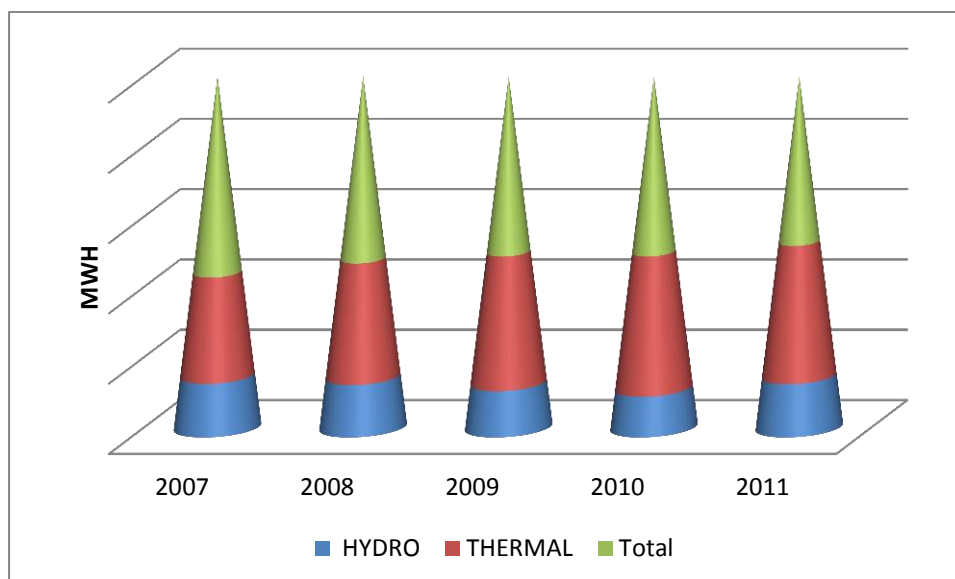
CHART 30: ELECTRICITY GENERATION, 2007 – 2011
