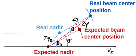
Figure B1. Definition of mispointing geometrical parameters \theta and \theta' . We recall that Z is the satellite altitude.
