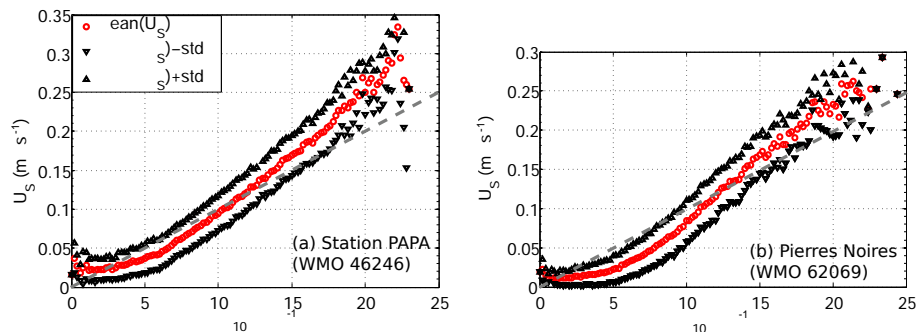
Figure 4. Example of mean value (in red) of the Stokes drift vector norm U_S = |\mathbf{U}_S| as a function of wind speed for two locations: station PAPA in the northeast Pacific, and buoy 62069 off the French Atlantic coast. The black symbols show the mean \pm 1 standard deviation for each wind speed. The dashed grey line is U_S = 0.01 U_{10} . This estimation covers only frequencies up to 0.58 Hz.
