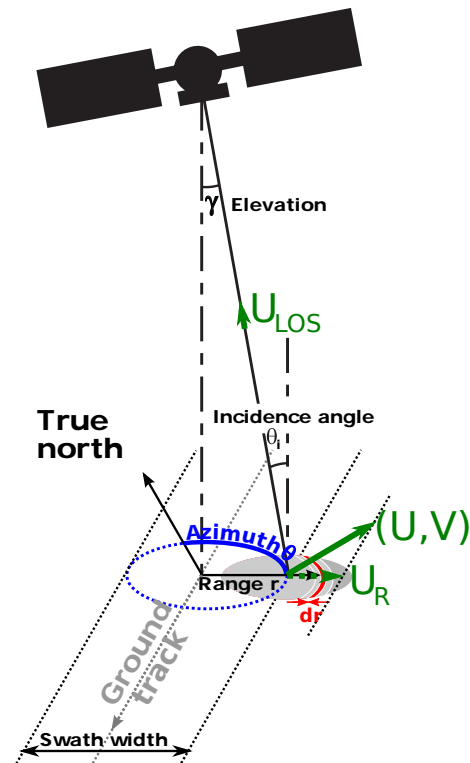
Figure 2. Geometry of measurement from a radar with a local incidence angle \theta_i , looking towards azimuth \theta_a . For simplicity of the schematic, we have taken U_{WB} = 0 and U_{NG} = 0 , so that the line-of-sight velocity is simply U_{LOS} = U \sin \theta_i + V \cos \theta_i / \sin \theta_i . Note that the diameter of the footprint (6 km) is exaggerated compared to the swath width (270 km) for readability. The small difference between elevation \gamma and incidence angle \theta_i is due to the Earth curvature.
