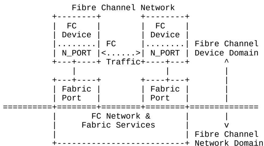
Figure 6. A Fibre Channel Network
