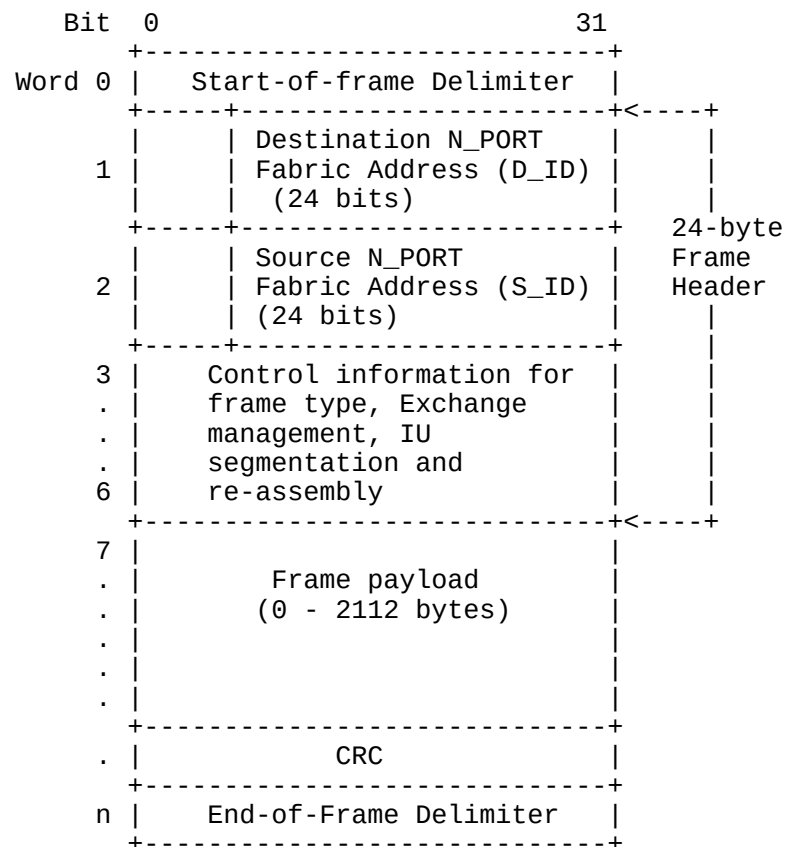
Figure 4. Fibre Channel Frame Format
