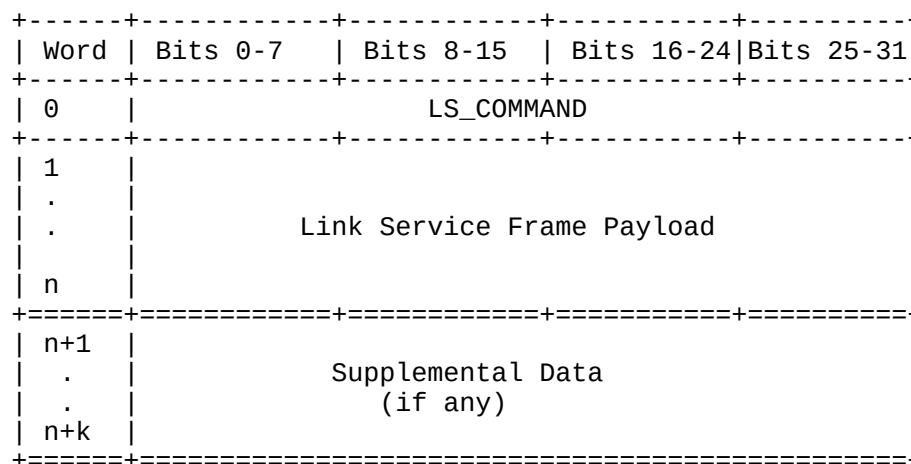
Figure 20. Special Link Service Frame Payload
