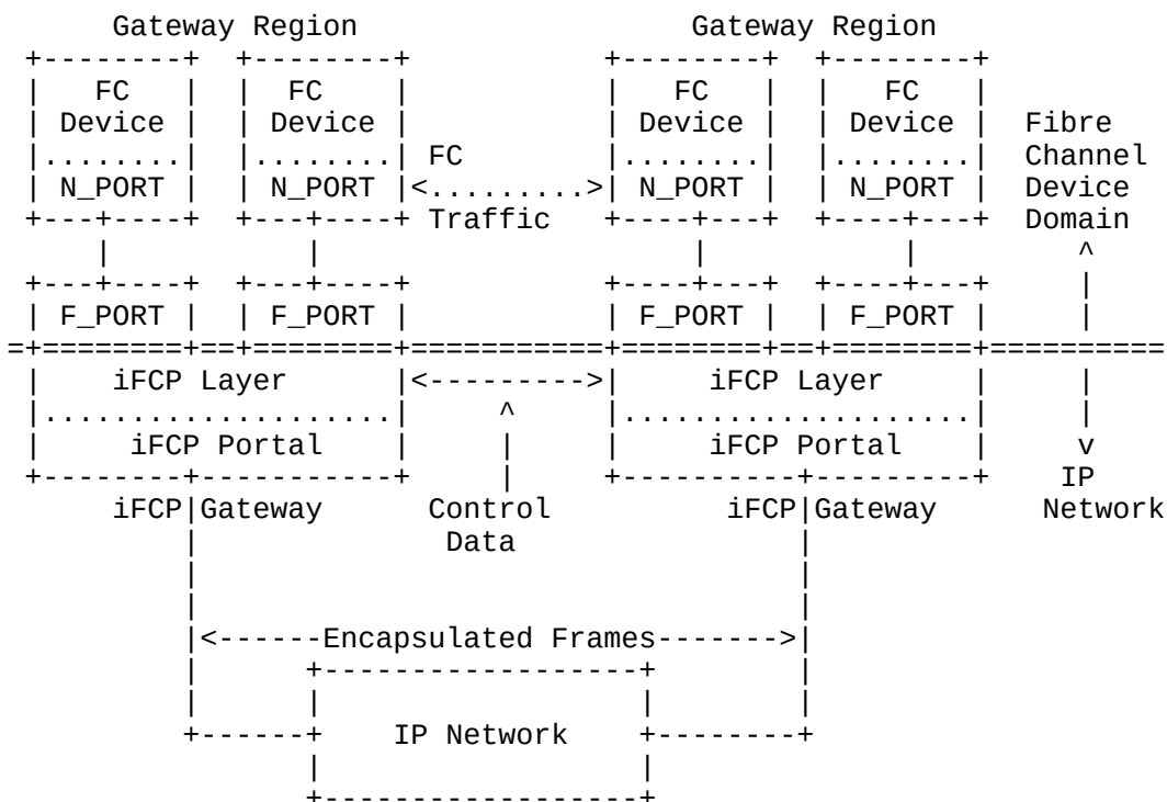
Figure 7. An iFCP Fabric Example
