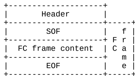
Figure 12. Encapsulation Format
