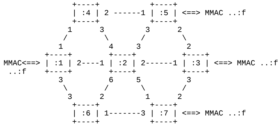
Figure 5: SPBV Example 7-Node Network
