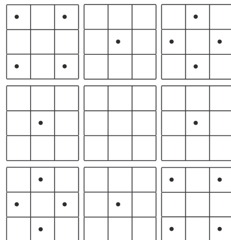
Figure 4. The four-dimensional space \mathbb{F}^4 is depicted as a 3 \times 3 grid of 3 \times 3 squares. The squares with dots represent the 20 vectors that form the Pellegrino cap
