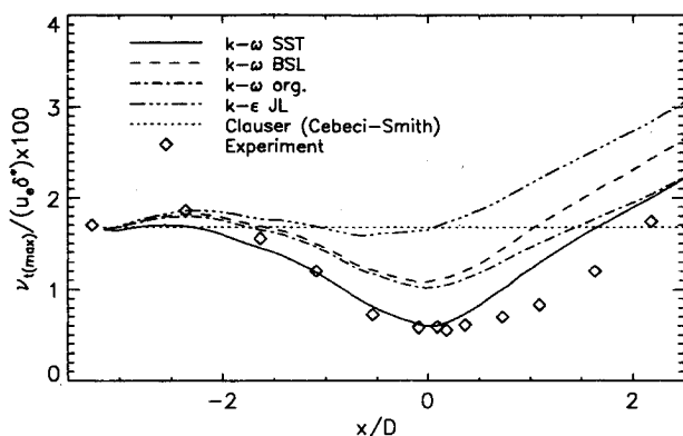
Fig. 6 \nu_t(max)/u_e \delta^* distribution for Driver's adverse pressure-gradient flow.
